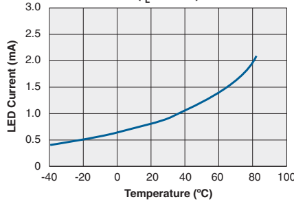
CPC1231N Typical I_F for Switch Operation vs. Temperature ( I_L=50mA )
